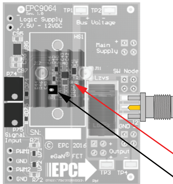
Figure 3: Proper measurement of the switch nodes.
