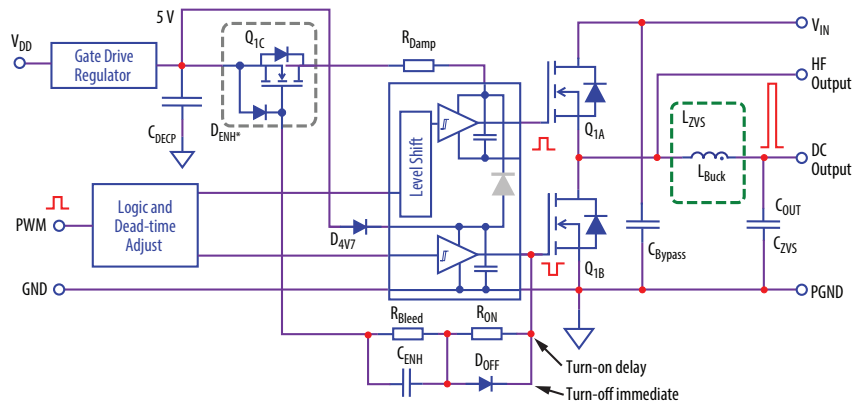
Figure 1: Block diagram of EPC9064 development board.
